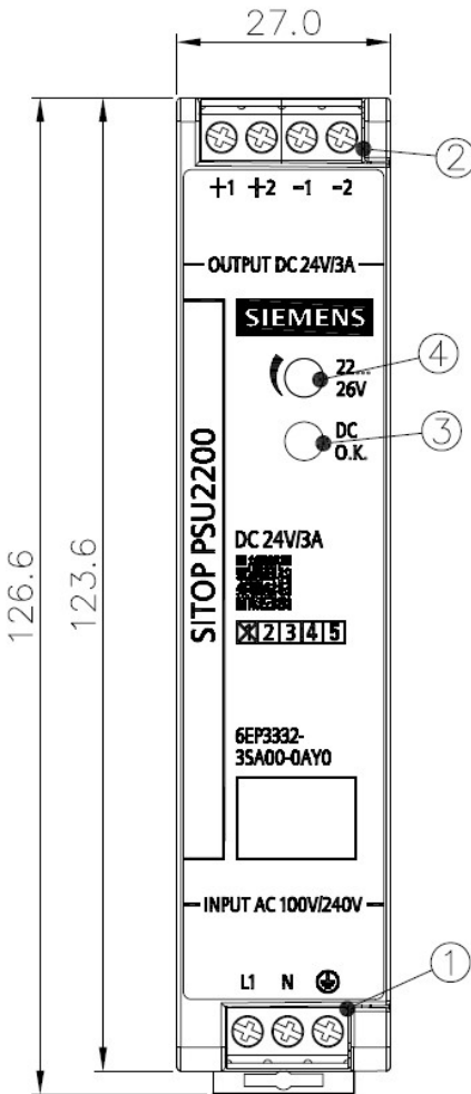
图 3: 结构 Figure 3: Structure
